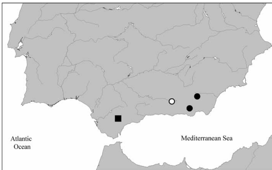
Map 4: Distributions of Oxyptoda telifera nov.sp. (square), O. imminuta nov.sp. (filled and open circles), and O. incurvata nov.sp. (open circle) in southern Spain.
