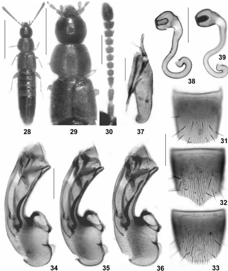
Figs 28-39: Oxyptoda virgata nov.sp.: (28) habitus; (29) forebody; (30) antenna; (31) male tergite VIII; (32) male sternite VIII; (33) female sternite VIII; (34-36) median lobe of aedeagus in lateral view; (37) paramere; (38-39) spermatheca. Scale bars: 28: 1.0 mm; 29: 0.5 mm; 30-33: 0.2 mm; 34-39: 0.1 mm.
