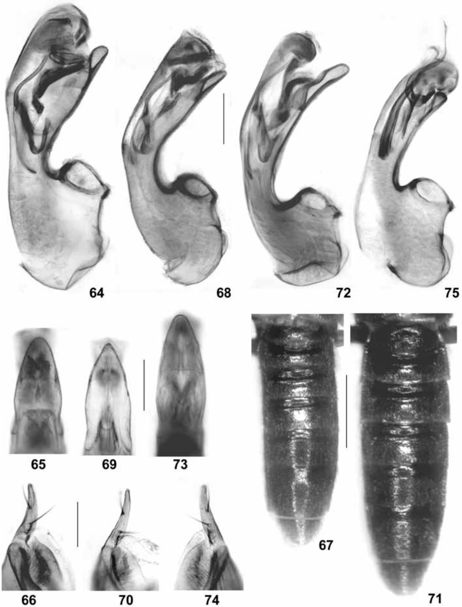
Figs 64-75: Oxypoda telifera nov.sp. (64-66), O. imminuta nov.sp. (67-70), O. incurvata nov.sp. (71-74), and O. haemorrhhoa (MANNERHEIM) (75): (64, 68, 72, 75) median lobe of aedeagus in lateral view; (65, 69, 73) apical portion of median lobe of aedeagus in ventral view; (66, 70, 74) apical lobe of paramere; (67, 71) abdomen. Scale bars: 67, 71: 0.5 mm; 64-66, 68-70, 72-75: 0.1 mm.
