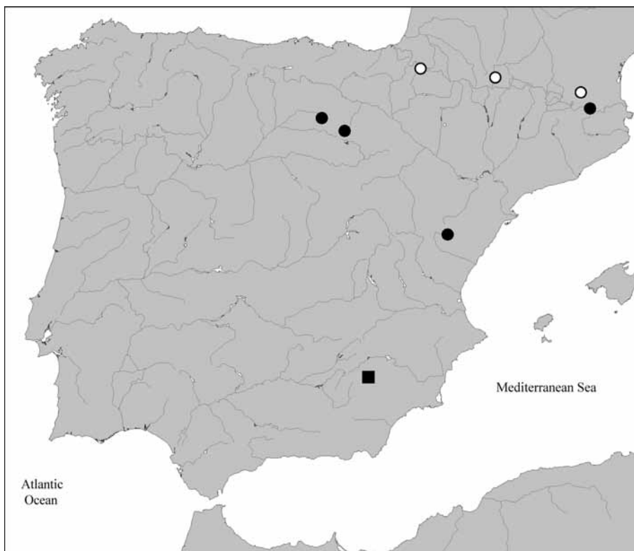
Map 1: Distribution of the species of the Proteinus crenulatus group in the Iberian Peninsula: P. crenulatus PANDELLÉ (open circles), P. hamatus ASSING (filled circles), and P. leincinai nov.sp. (square).
